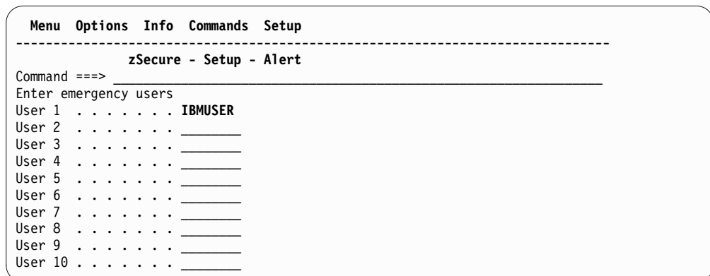
Figure 22. Setup Alert panel: Configuring emergency users (alerts 1102 and 2102) panel
